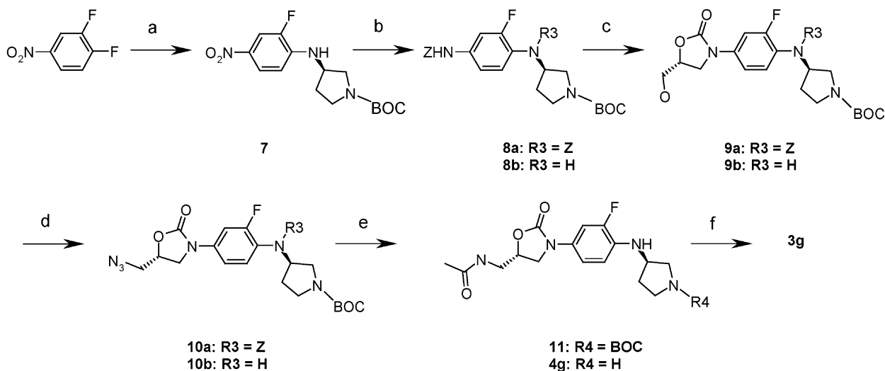
Scheme 2. (a) (1) 3( R )-1-Allyloxycarbonyl-3-amino-pyrrolidine, Et 3 N; (2) PdCl 2 (PPh 3 ) 2 , AcOH, Bu 3 SnH; (3) BOC 2 O; (b) (1) H 2 , Pd/C; (2) ZCl, NaHCO 3 ; (c) n -BuLi, R -(-)-glycidyl butyrate; (d) (1) MsCl, TEA; (2) NaN 3 ; (e) (1) H 2 , Pd/C; (2) Ac 2 O, AcOH; (3) Et 3 SiH, TFA; (f) 5a (Y = CH; R 2 = cyclopropyl), DABCO.
