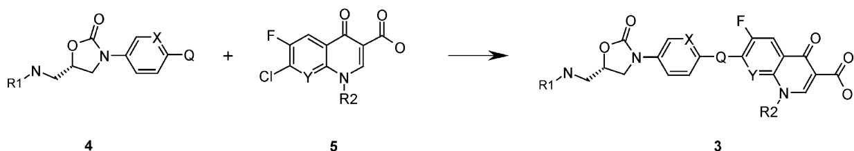
Scheme 1. Strategy for the assembly of the oxazolidinone–quinolone hybrids 3 .
